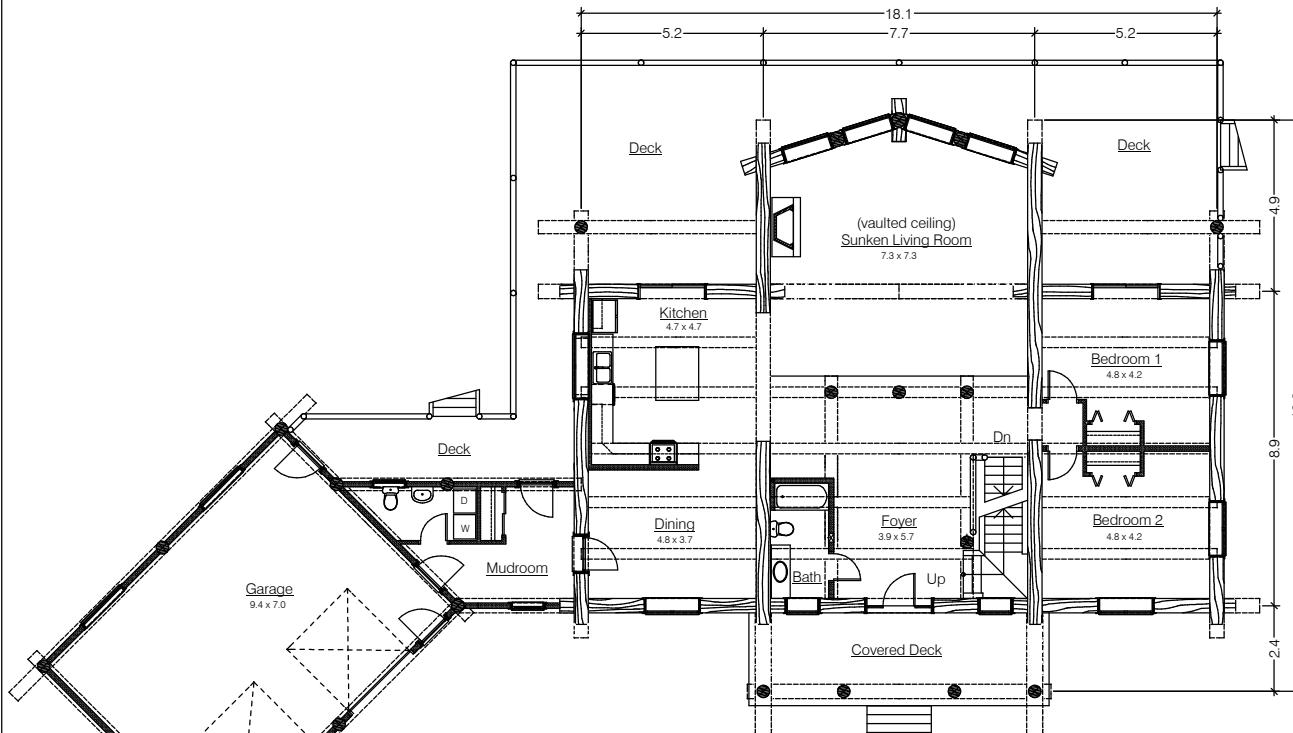
Main Floor Plan House - 219.5 Sq. M. Garage - 71.3 Sq. M.
